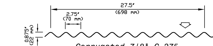
Corrugated 7/8" C-275
